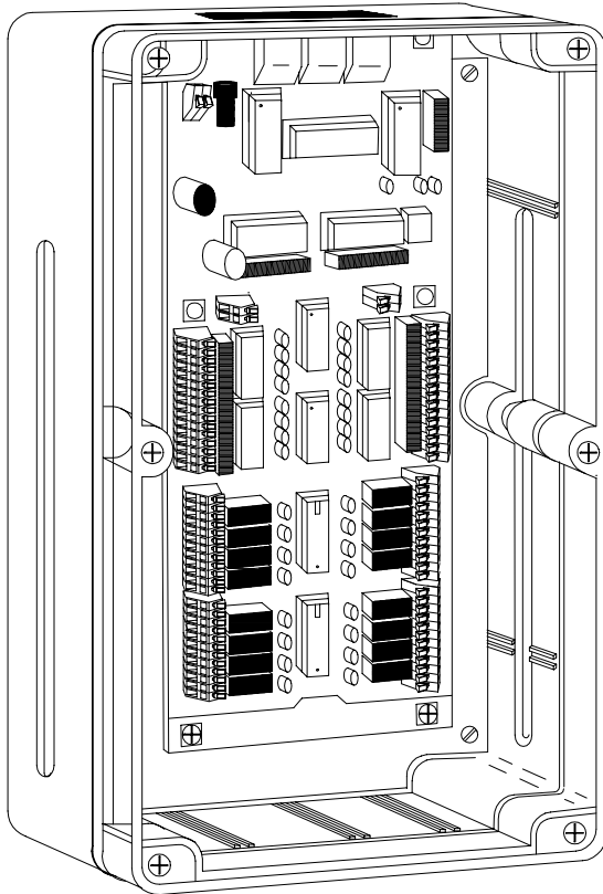
OPTIONAL ENCLOSURE FOR USN1616L, USN88ANL AND OTHER ANALOG AND/OR DIGITAL DISTRIBUTED UNITS. $45.00 EA.
